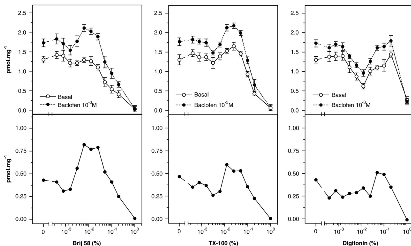
Fig. 6. Detergent effect on the baclofen-stimulated [ ^{35} S]GTP \gamma S binding in brain cortex PM. The upper panels depict the activity of the basal (○) and baclofen-stimulated (●) [ ^{35} S]GTP \gamma S binding. The bottom panels show the difference between the baclofen-stimulated and basal [ ^{35} S]GTP \gamma S binding. PM fraction was mixed at 0–4 °C with increasing concentrations of Brij58 (right panel) or Triton X-100 (middle panel) to achieve the final concentration of 0.0004, 0.0008, 0.0016, 0.0031, 0.0063, 0.0125, 0.025, 0.05, 0.1, 0.2 and 1.0%; subsequently, an aliquot of membrane-detergent mix was transferred to [ ^{35} S]GTP \gamma S binding assay medium and incubated at 25 °C for 30 min with [ ^{35} S]GTP \gamma S as described in Materials and methods. Concentrated solution of Digitonin in DMSO (12%) was added to PM to achieve the same final concentration as in the case of the two water-soluble detergents (0.0004, 0.0008, 0.0016, 0.0031, 0.0063, 0.0125, 0.025, 0.05, 0.1, 0.2 and 1.0%), aliquots of membrane-detergent mix were transferred to [ ^{35} S]GTP \gamma S binding assay medium and incubated at 25 °C for 30 min as in the case of Brij58 and Digitonin. Results represent the average of 3 experiments \pm SEM.
