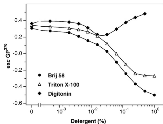
Fig. 3. The effect of detergents on the excitation generalized polarization GP_{exc} of Laurdan embedded in PM. Dependence of GP_{exc} of Laurdan on the concentration of Brij58 (●), Triton X-100 (Δ), and Digitonin (◆) was measured at the excitation wavelength of 370 nm in PM and GP_{exc} values were calculated as described in Materials and methods.
